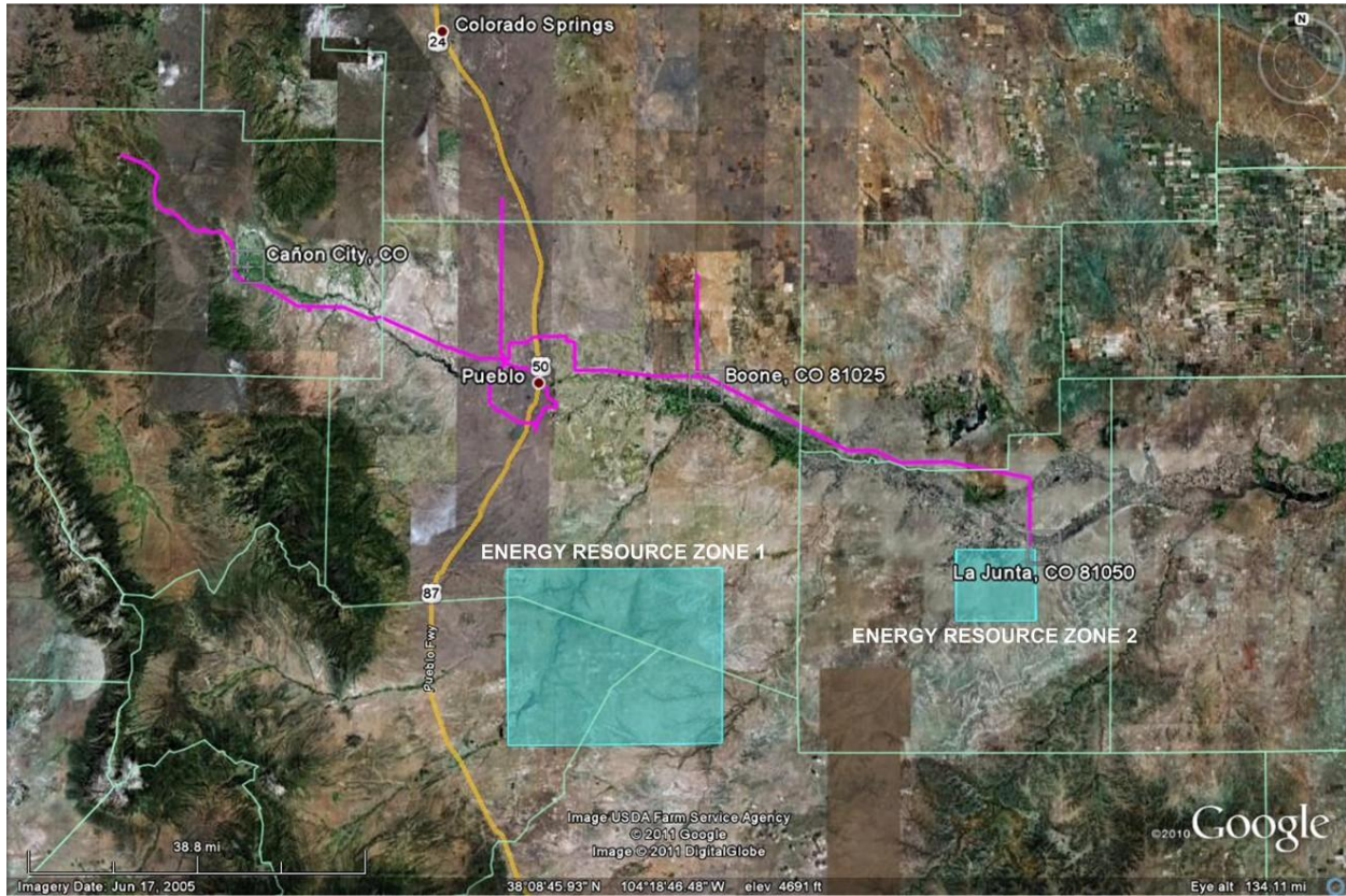
Figure 1: BHCE 115 kV Transmission System and ERZ
